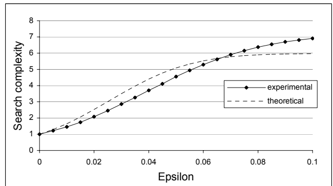
Fig. 4. Search complexity as a function of \epsilon .
