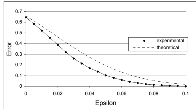
Fig. 3. Read error as a function of \epsilon .
