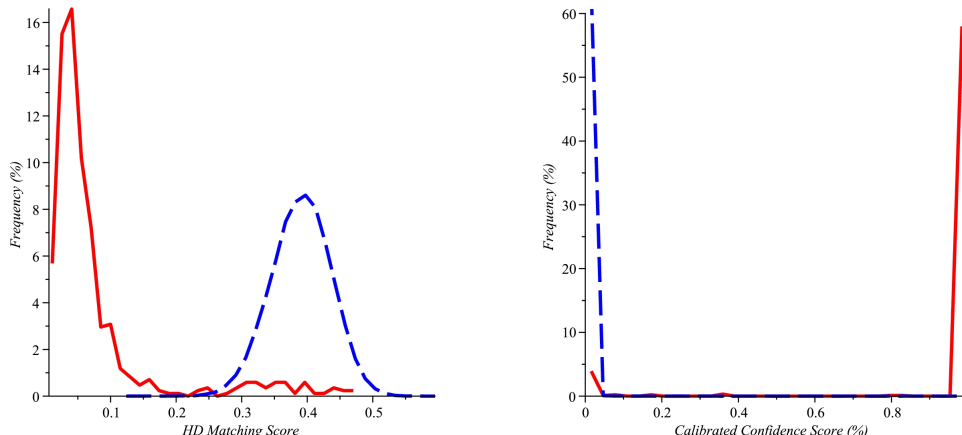
Figure 1: Genuine (solid line) and Impostor (dashed line) distributions of the matching scores and the calibrated confidence scores.
